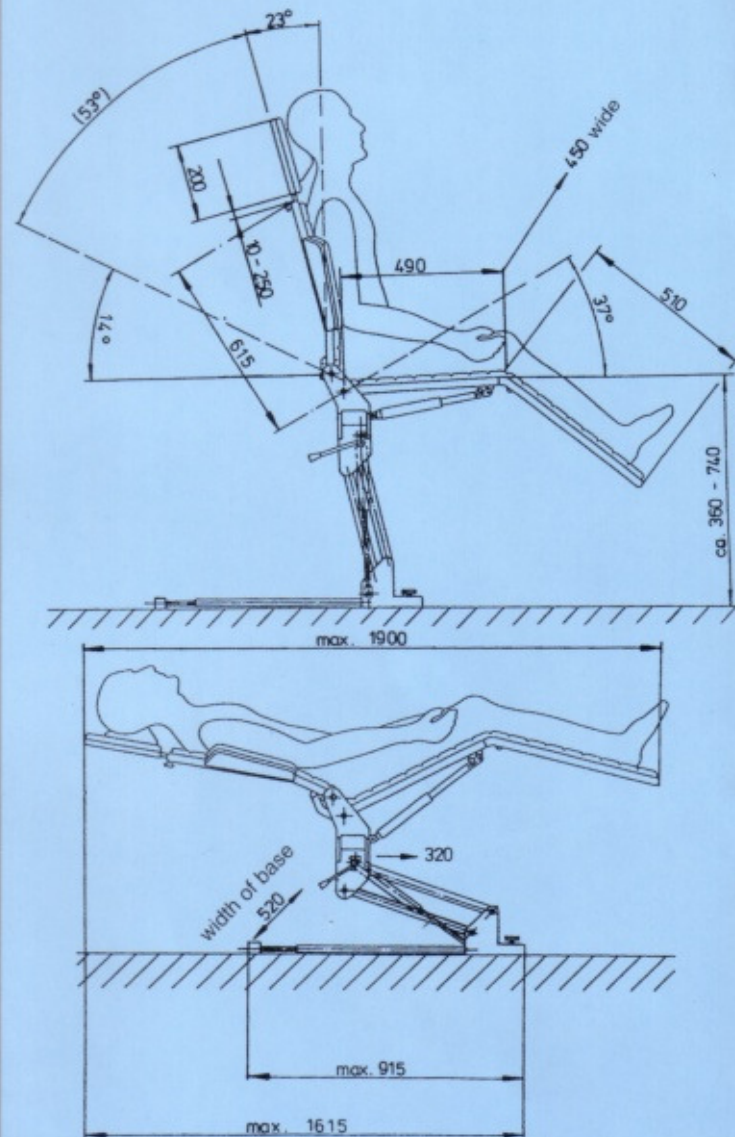
Patient chair no. 6140-00-00-dimensioned drawing
